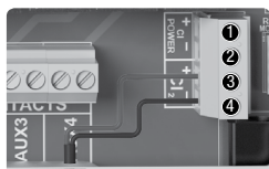
Free Chlorine probe ③ red ④ black
