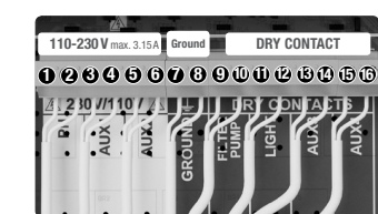
AUX 1 3 & 4 Base (pump) or Ultraviolet (according to model)
